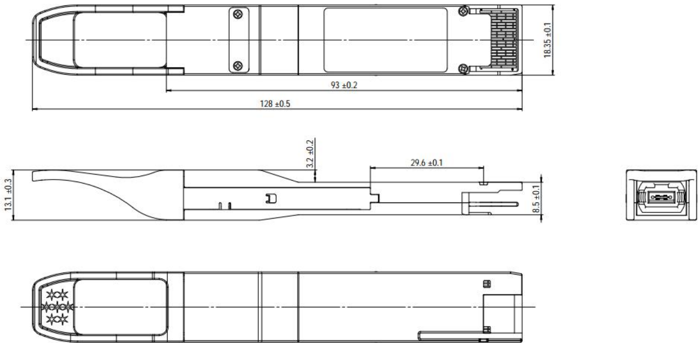
Figure10. Mechanical Specifications
