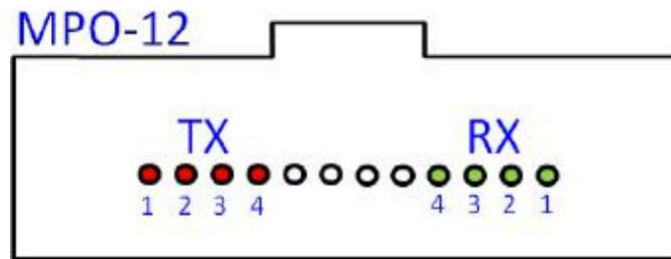
Figure 4. Optical Receptacle and Channel Orientation
