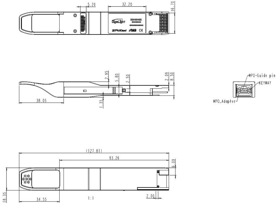
Figure6. Mechanical Specifications
