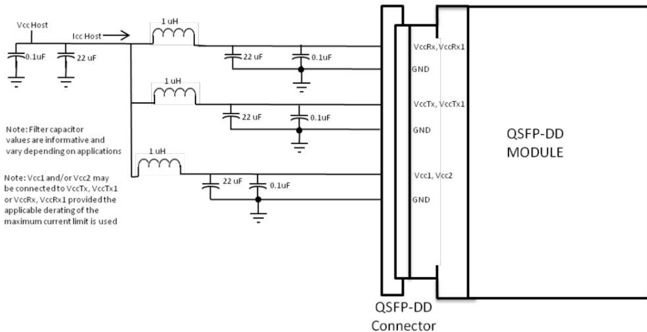
Figure 11. Host Board Power Supply Filtering
