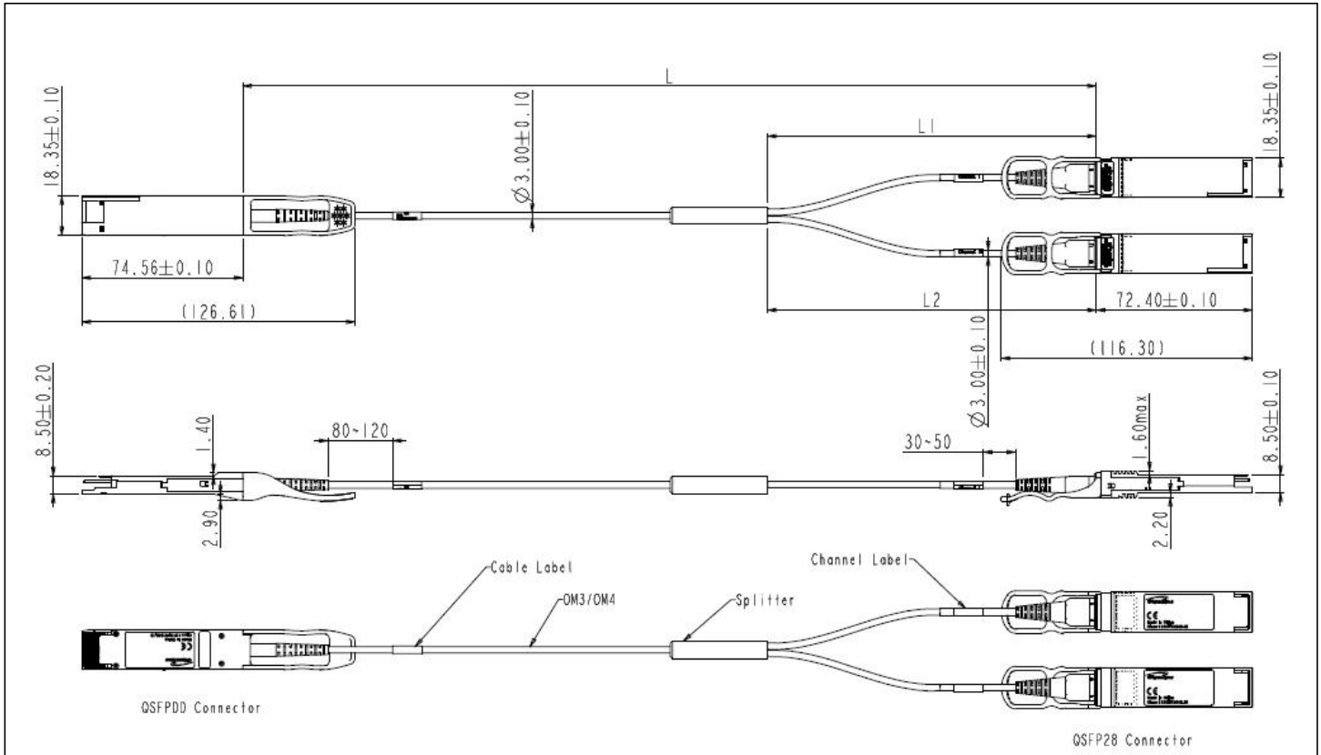
Figure 16. AOC Mechanical Specifications
