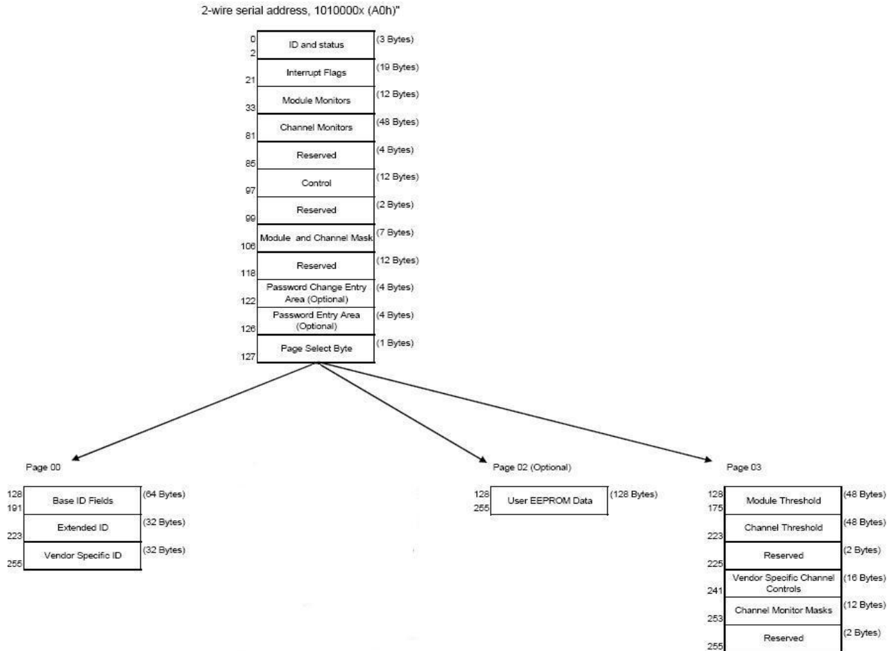
Figure6. QSFP Memory Map
