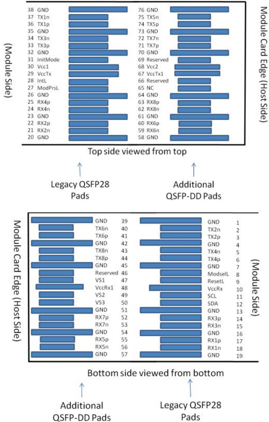
Figure 10. Electrical Pin-out Details
