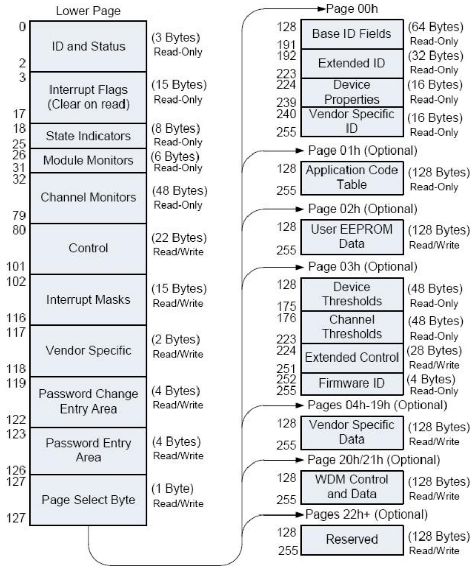
Figure 12. QSFP DD Memory Map
