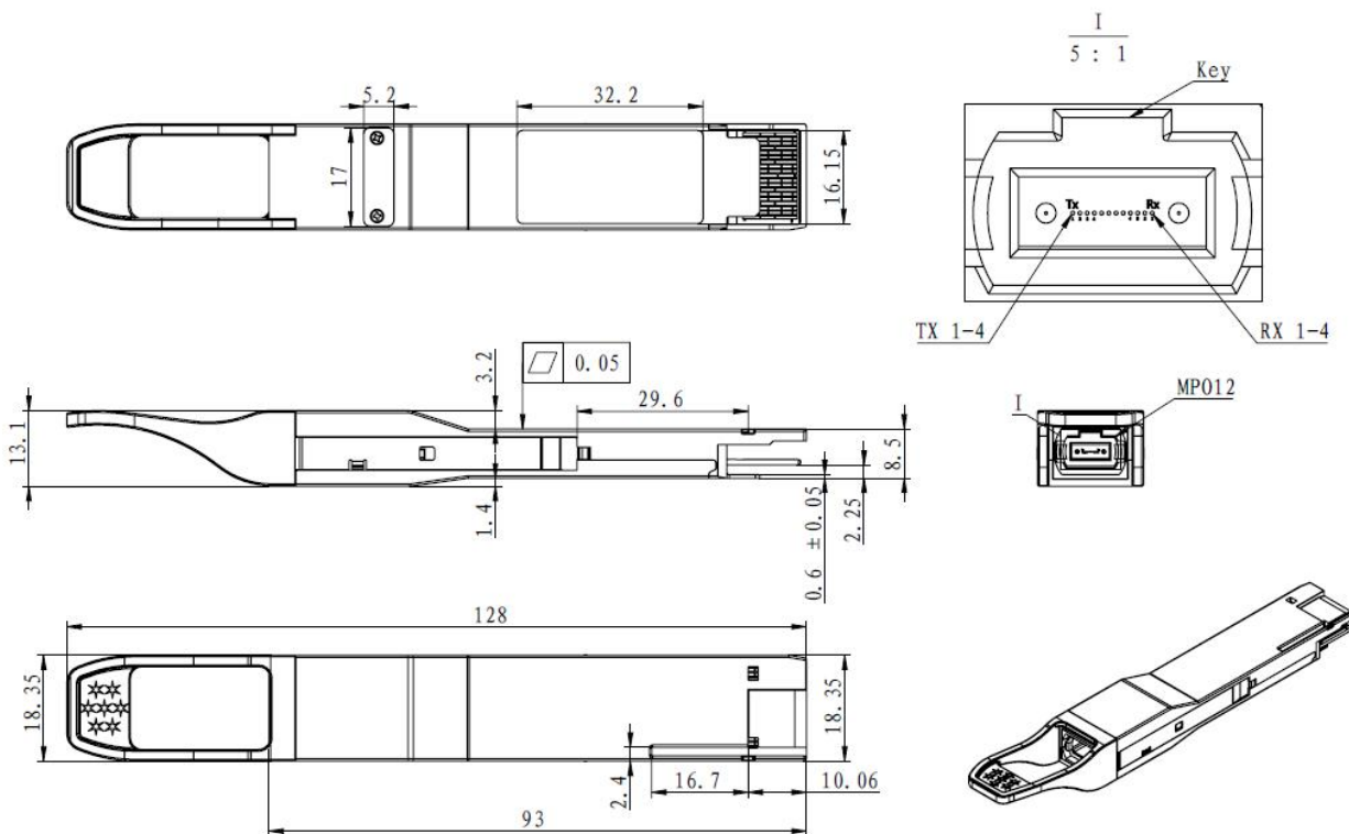
Figure5. Mechanical Specifications
