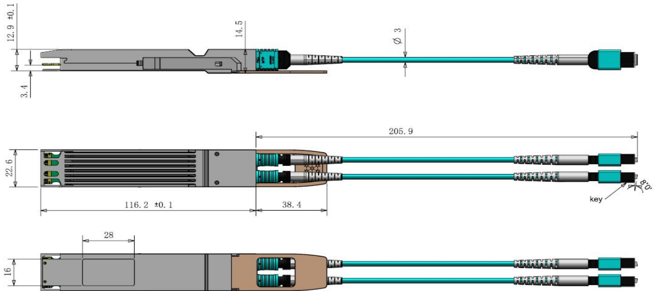
Figure7. Mechanical Specifications
