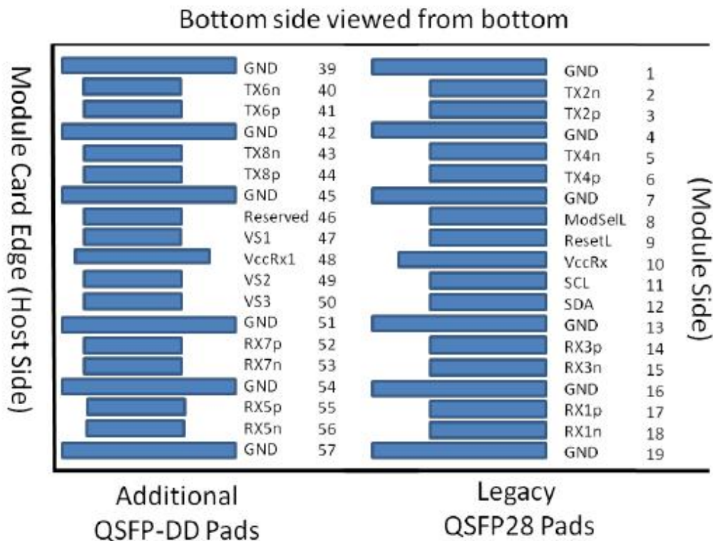
Figure3. Electrical Pin-out Details
