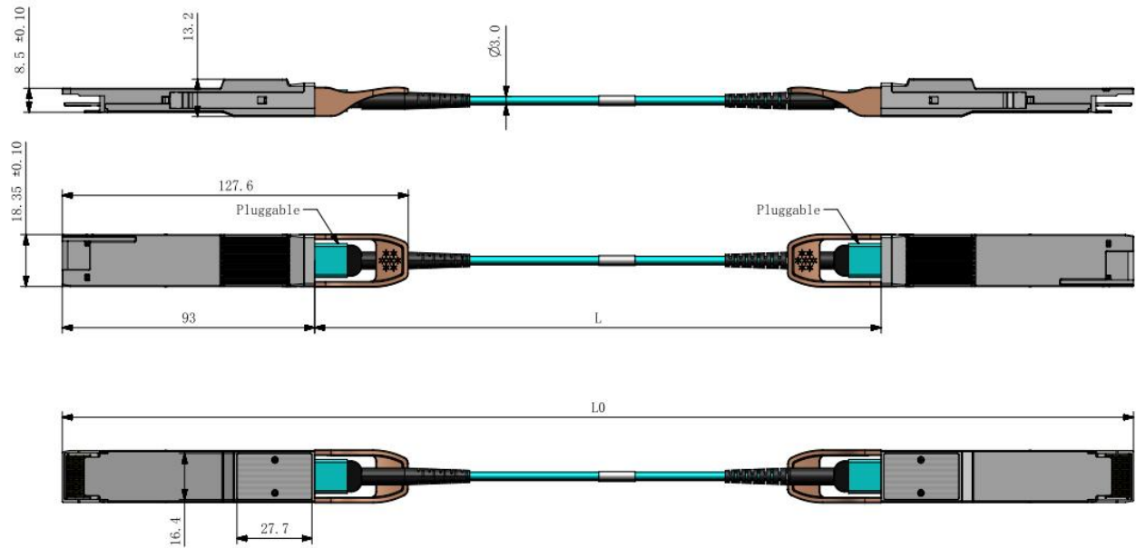
Figure7. Mechanical Specifications
